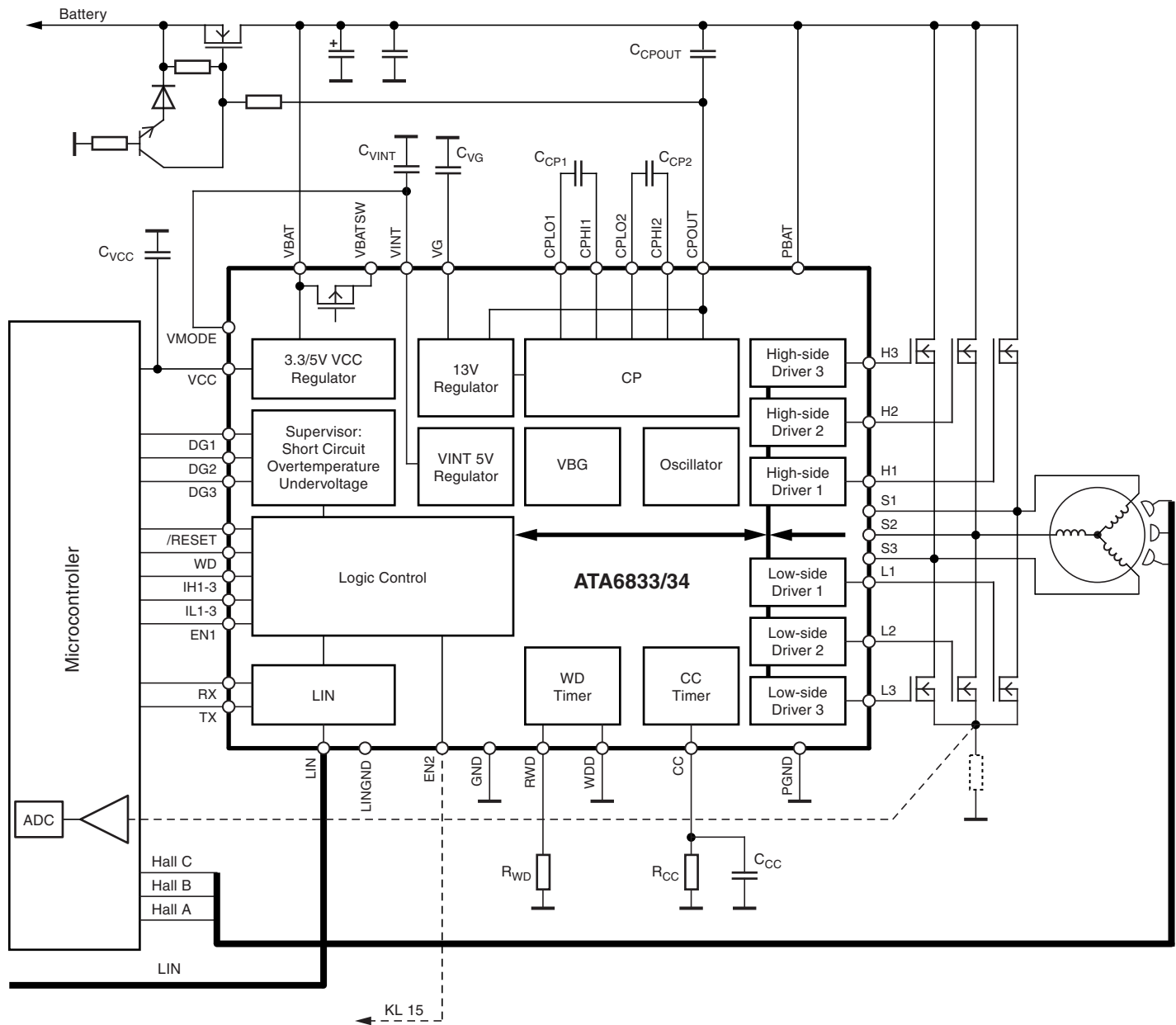
Figure 9-1. Typical Application
