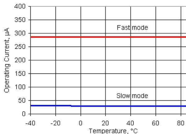
Figure 11-32. IDAC Operating Current vs Temperature, Range = 255 \mu\text{A} , Code = 0, Source Mode
