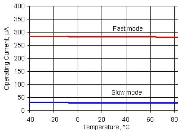
Figure 11-33. IDAC Operating Current vs Temperature, Range = 255 \mu\text{A} , Code = 0, Sink Mode
