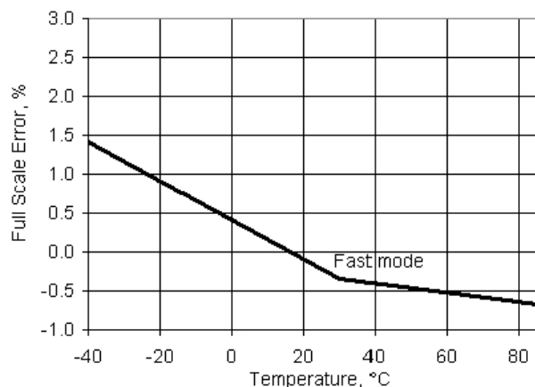
Figure 11-30. IDAC Full Scale Error vs Temperature, Range = 255 \mu\text{A} , Source Mode
