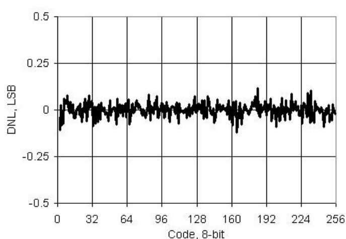
Figure 11-38. VDAC DNL vs Input Code, 1 V Mode
