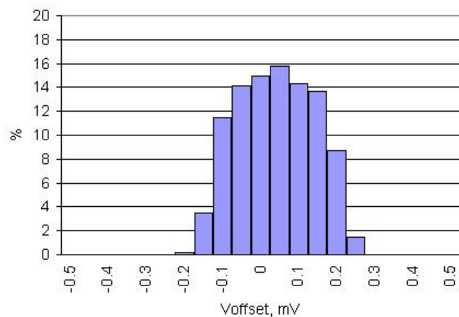
Figure 11-16. Opamp Voffset Histogram, 3388 samples/847 parts, 25\text{ }^{\circ}\text{C} , V_{DDA} = 5\text{ V}
