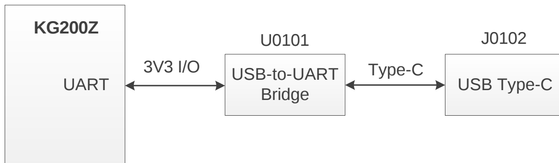
Figure 10: USB-to-UART Connection
