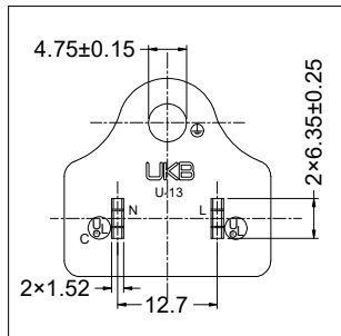
PLUG DETAILS
