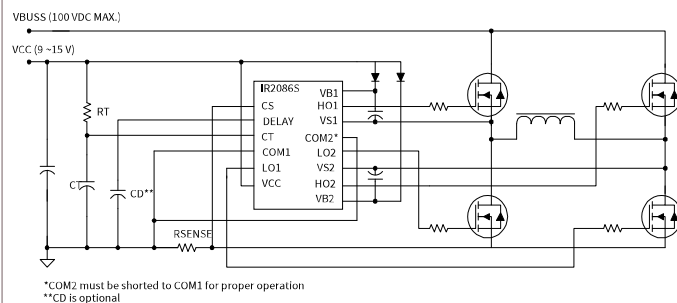
Typical connection
