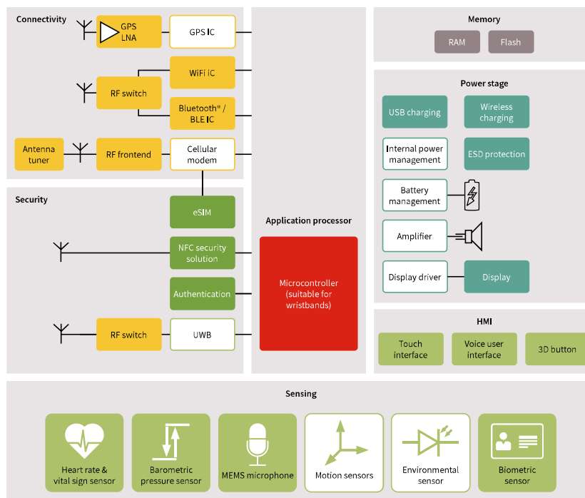
Block diagram for smartwatch, sports watch and wristband
