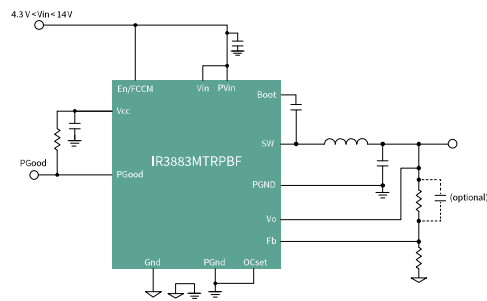
Block diagram IR3883M
