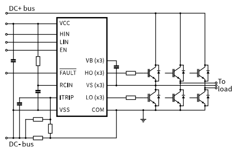
Typical connection
