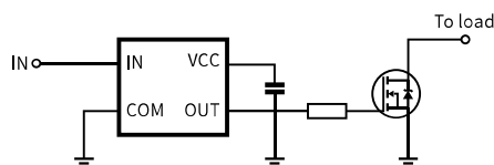
Typical connection
