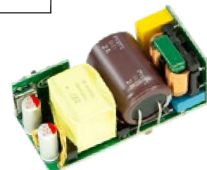
Infineon's 20 W/in 3 adapter (cased) - 24 W/in 3 (uncased) with 65 W output power capability (LxWxH: 74.2 mm x 36.5 mm x 16.5 mm)
