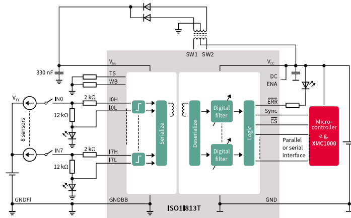
Digital input switch block diagram
