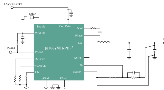
Block diagram IR3887M (30 A)
