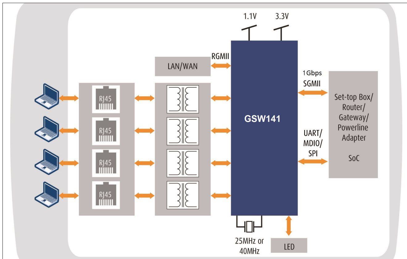
Figure 3 Home Gateway
