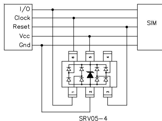
Figure 6 - SIM Port
