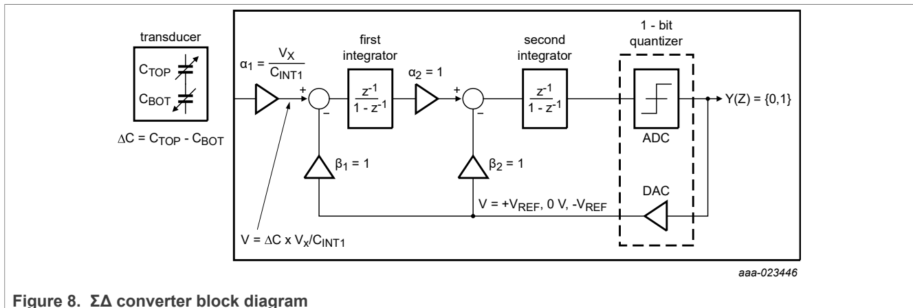
Figure 8. ΣΔ converter block diagram
