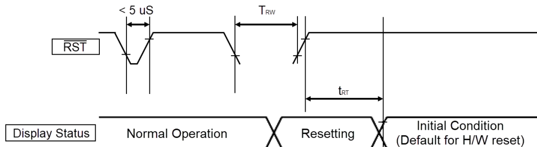
Figure 4: Reset Timing
