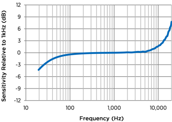
Figure 6: Typical Free Field Magnitude and Masks
