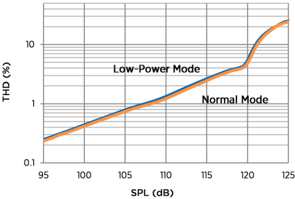
Figure 7: Typical THD vs SPL
