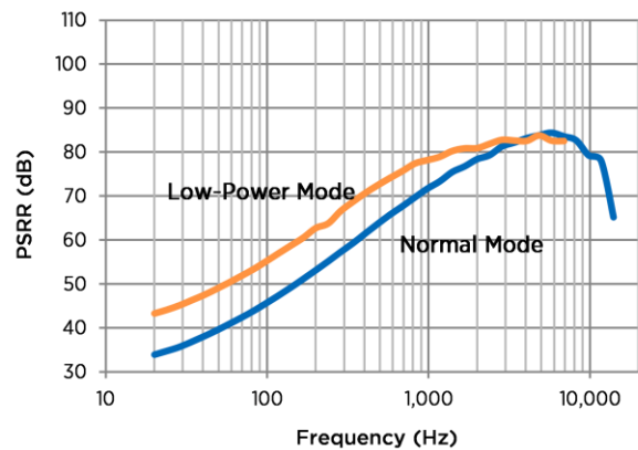
Figure 13: Typical PSRR
