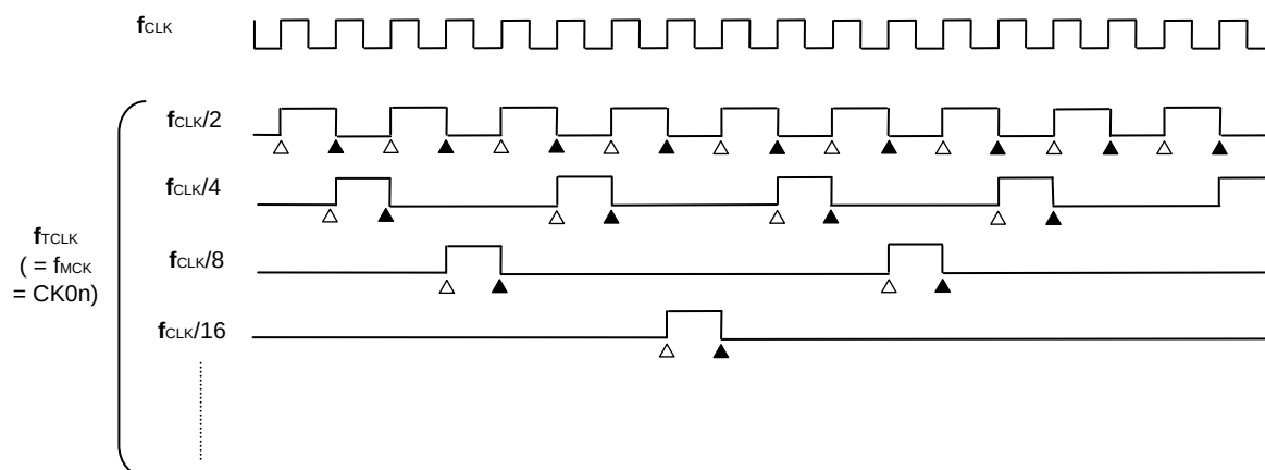
Figure 6-31. Timing of f_{\text{CLK}} and count clock ( f_{\text{CLK}} ) (When CCS0n = 0)
