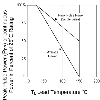
FIGURE 3 - Derating Curve
