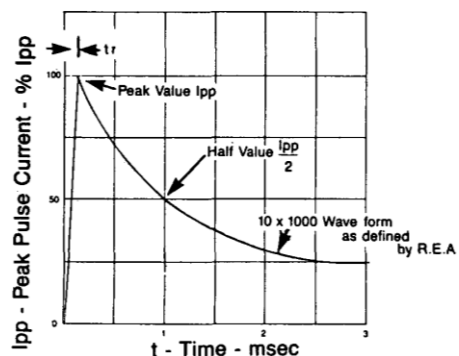
FIGURE 2 - Pulse waveform
