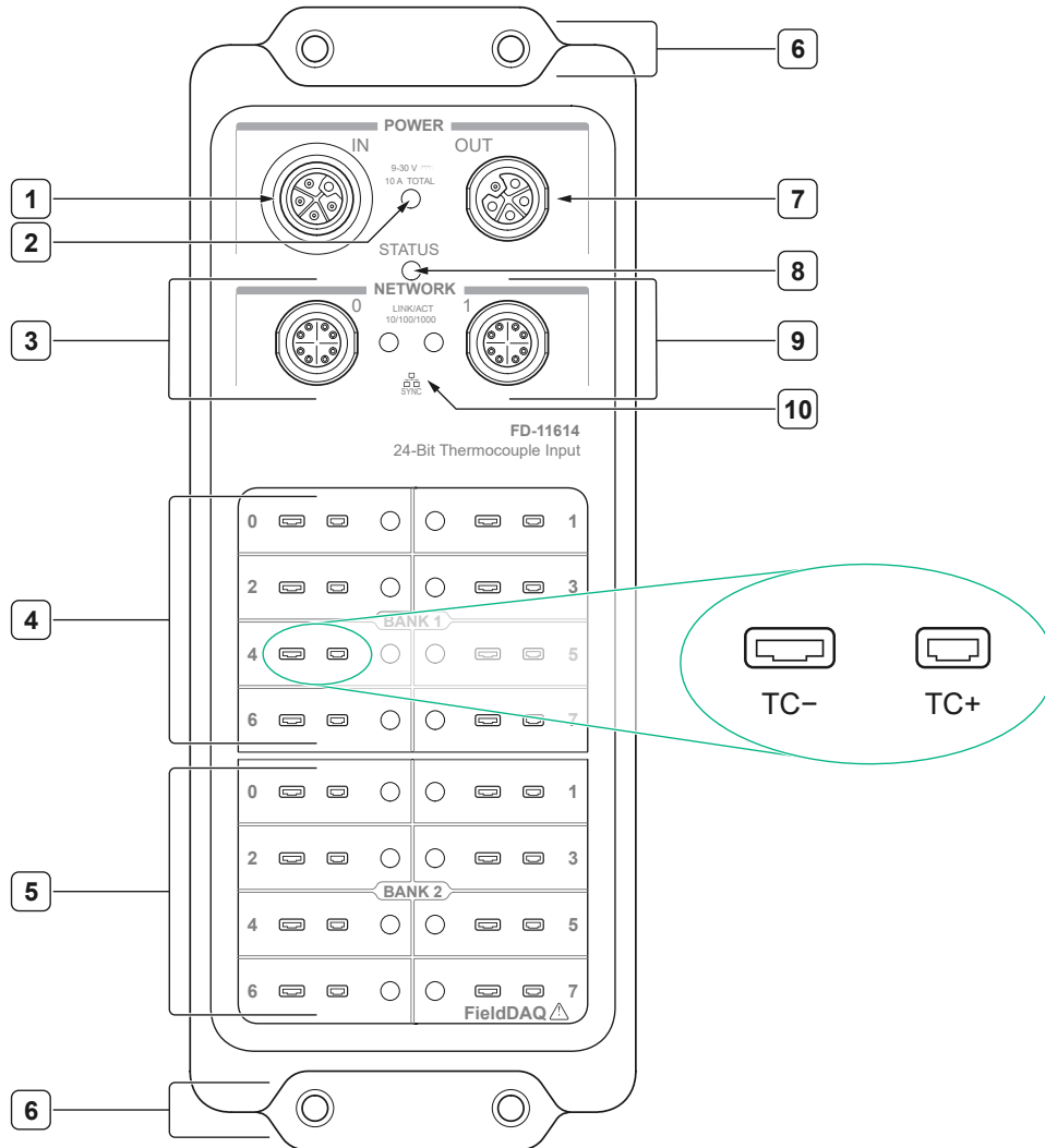
Figure 1. FD-11614 Front Panel
