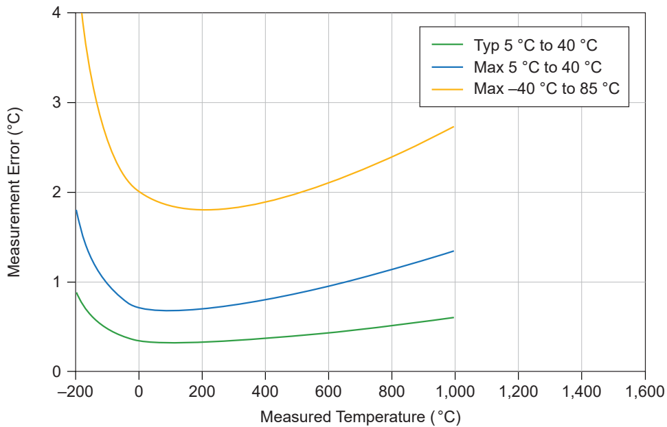
Figure 14. Thermocouple Type E Errors (High Speed)
