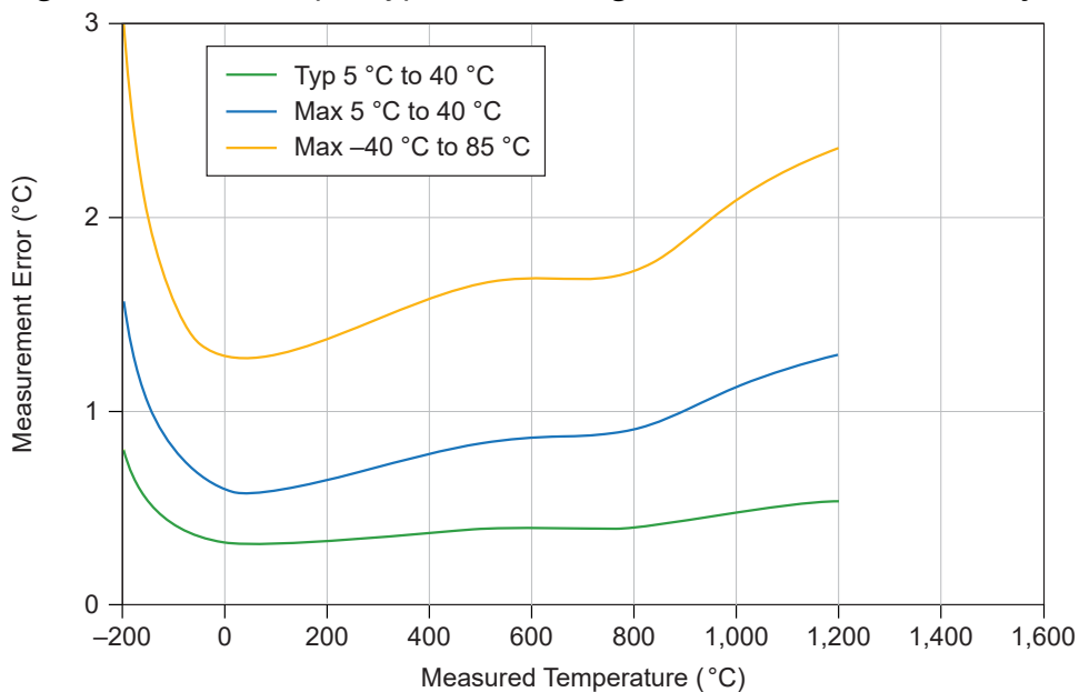
Figure 7. Thermocouple Type J Errors (High Resolution/Best 50 Hz Rejection/Best 60 Hz Rejection)
