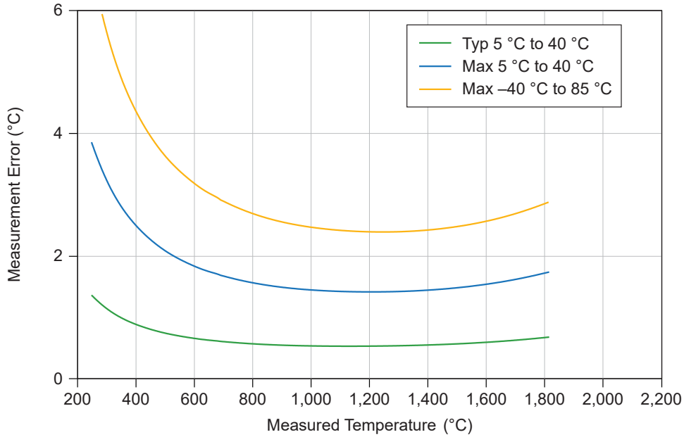
Figure 16. Thermocouple Type B Errors (High Speed)
