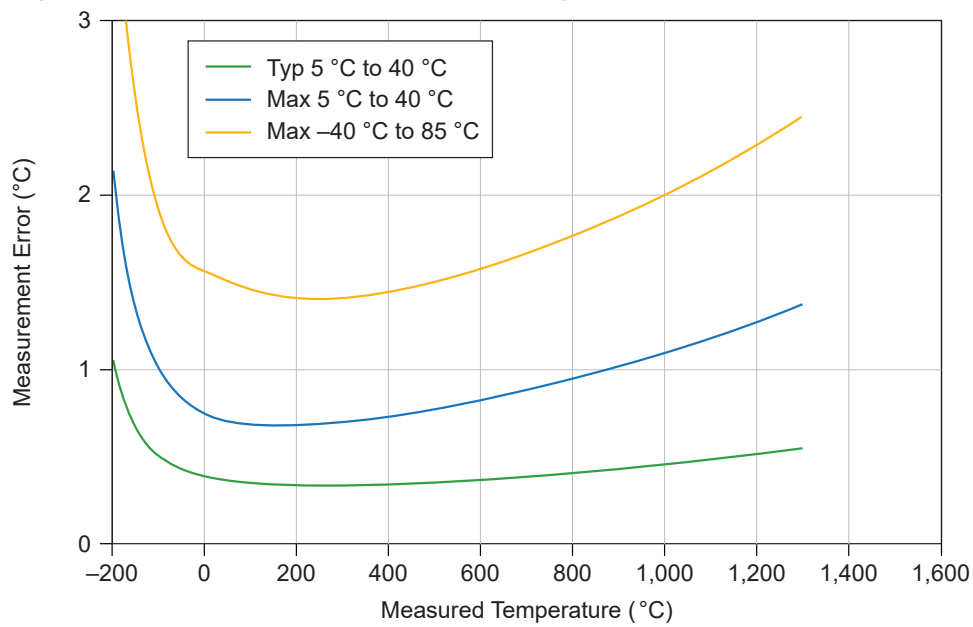
Figure 10. Thermocouple Type N Errors (High Speed)
