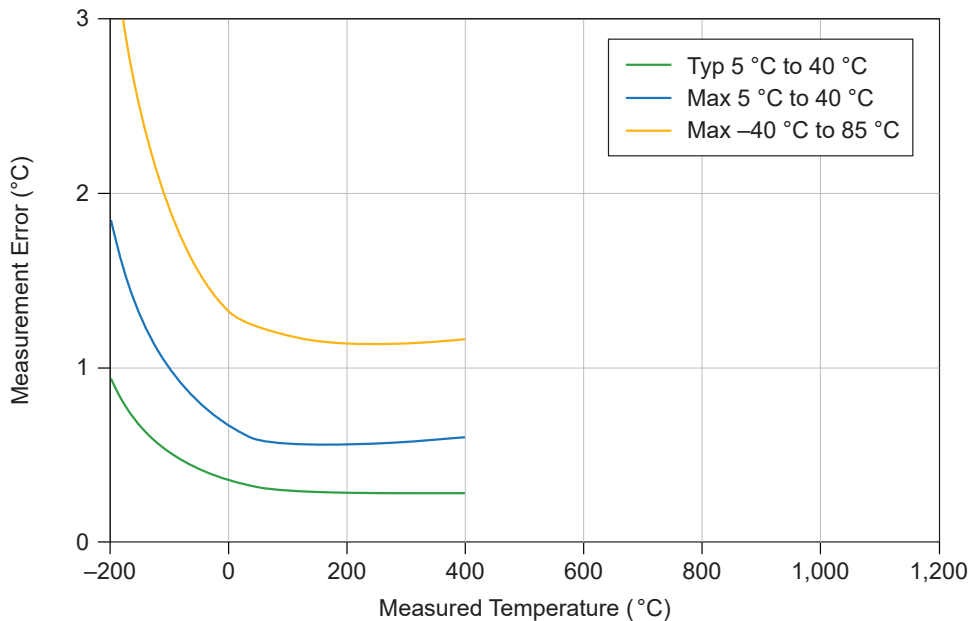
Figure 11. Thermocouple Type T Errors (High Resolution/Best 50 Hz Rejection/Best 60 Hz Rejection)
