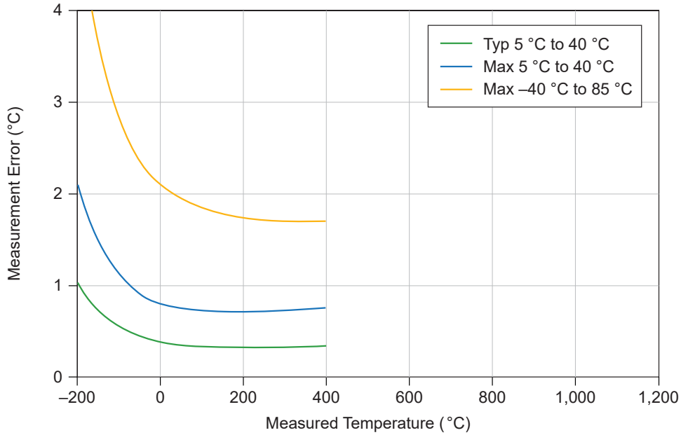
Figure 12. Thermocouple Type T Errors (High Speed)
