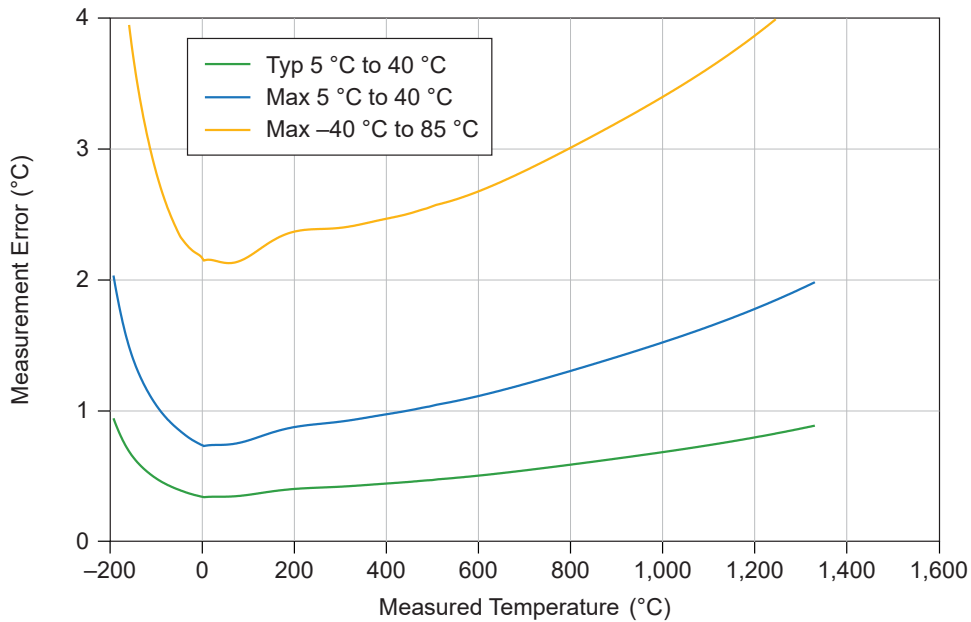
Figure 6. Thermocouple Type K Errors (High Speed)
