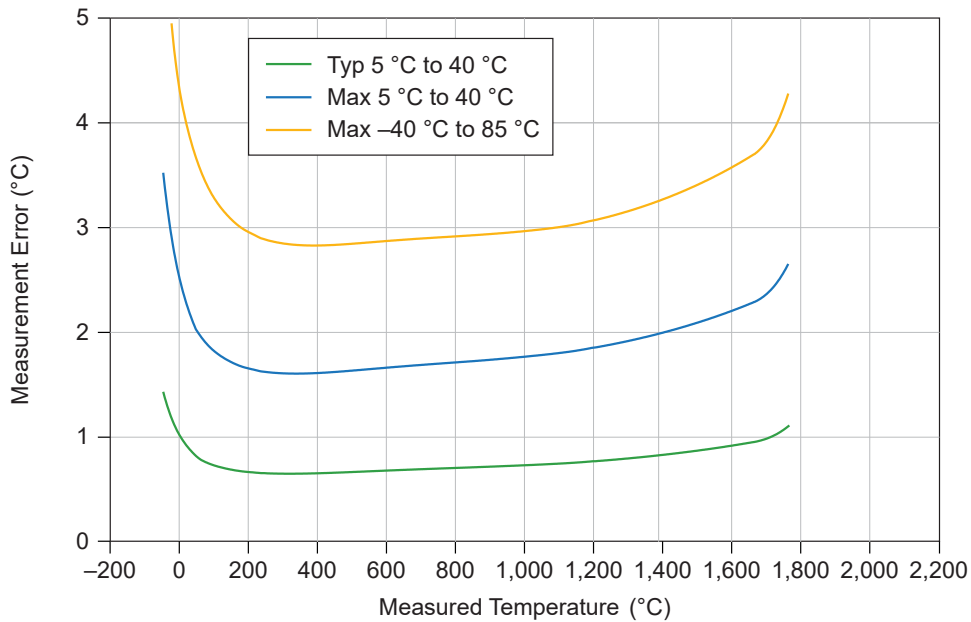
Figure 18. Thermocouple Type R/S Errors (High Speed)
