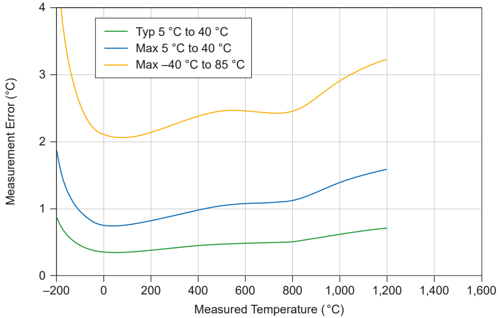
Figure 8. Thermocouple Type J Errors (High Speed)
