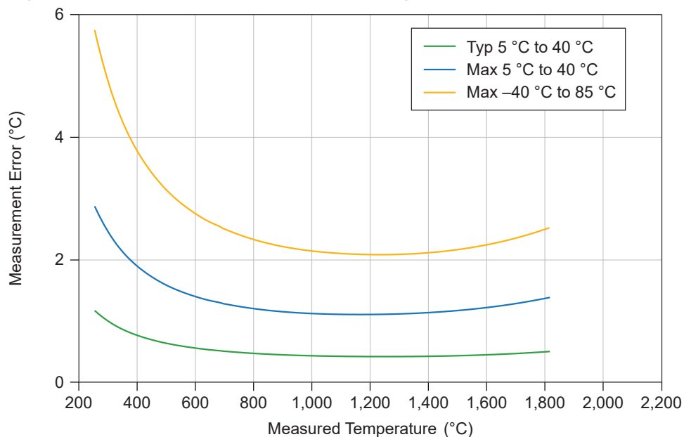
Figure 15. Thermocouple Type B Errors (High Resolution/Best 50 Hz Rejection/Best 60 Hz Rejection)
