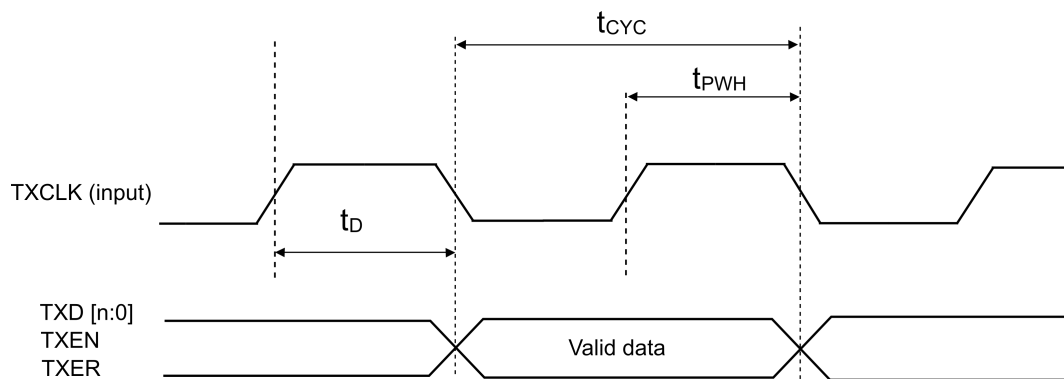
Figure 47. MII Transmit Timing
