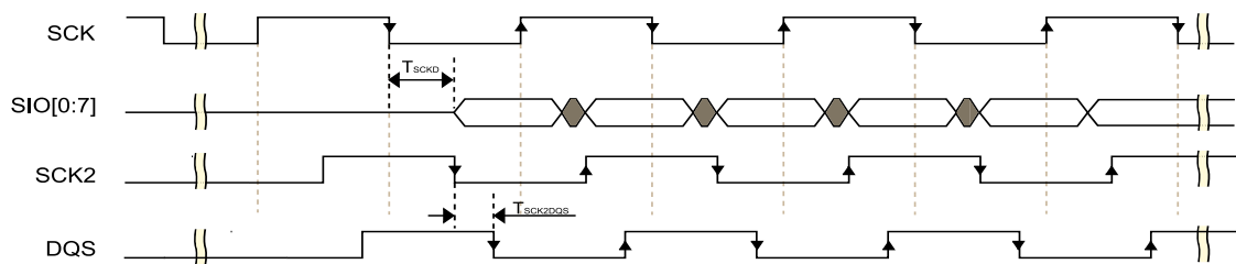
Figure 18. FlexSPI input timing in DDR mode where FlexSPI n _MCR0[RXCLKSRC] = 0x3 (caseB2)
