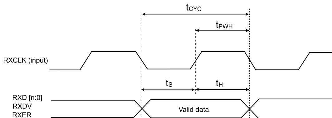
Figure 46. MII Receive Timing
