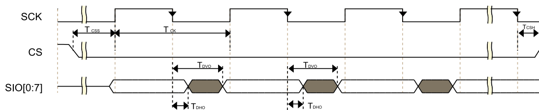
Figure 19. FlexSPI output timing in SDR mode
