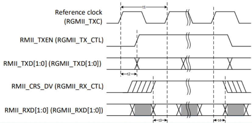
Figure 48. RMII timing diagram
