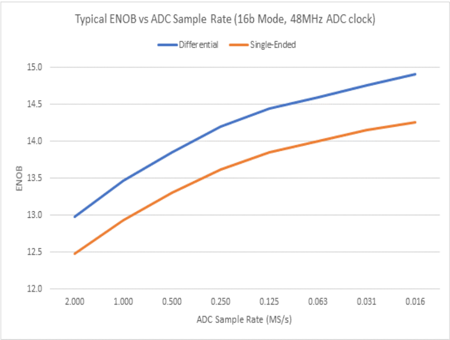
Figure 22. ENOB VS ADC clock graph
