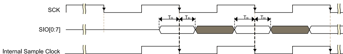
Figure 13. FlexSPI input timing in SDR mode where FlexSPI 1 _MCR0[RXCLKSRC] = 0x0 or 0x1 or 0x2
