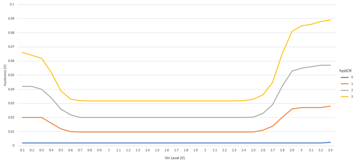
Figure 27. Typical hysteresis vs. Vin level (VDD = 3.3 V, HPMD = 1)
