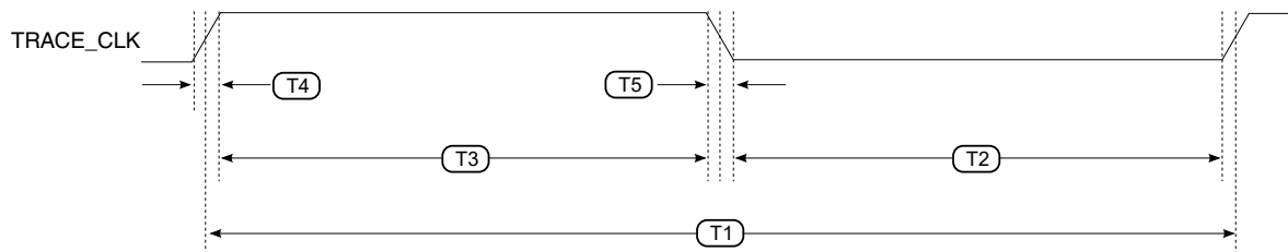
Figure 5. TRACE_CLKOUT specifications
