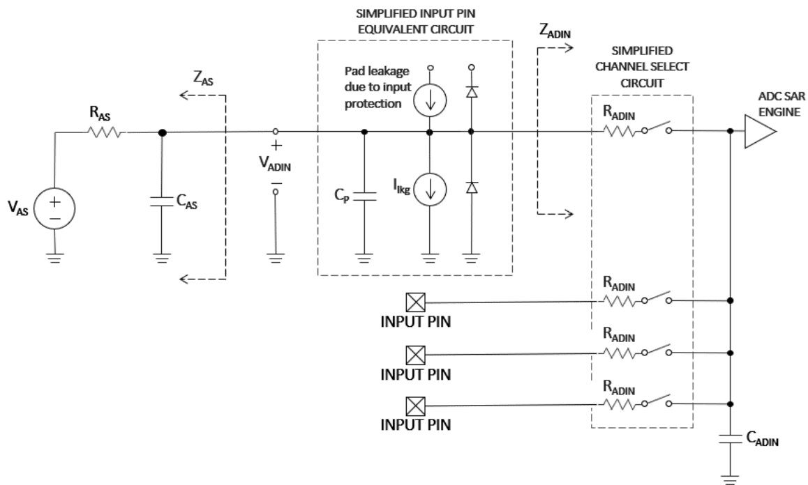
Figure 21. ADC input impedance equivalency diagram
