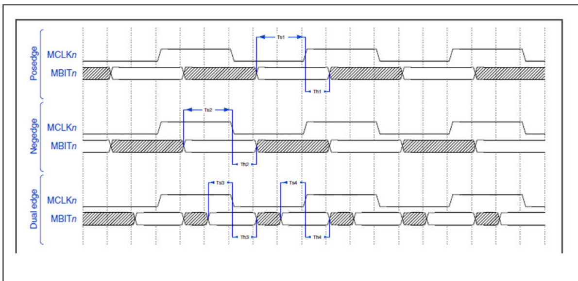
Figure 39. SINC timing
