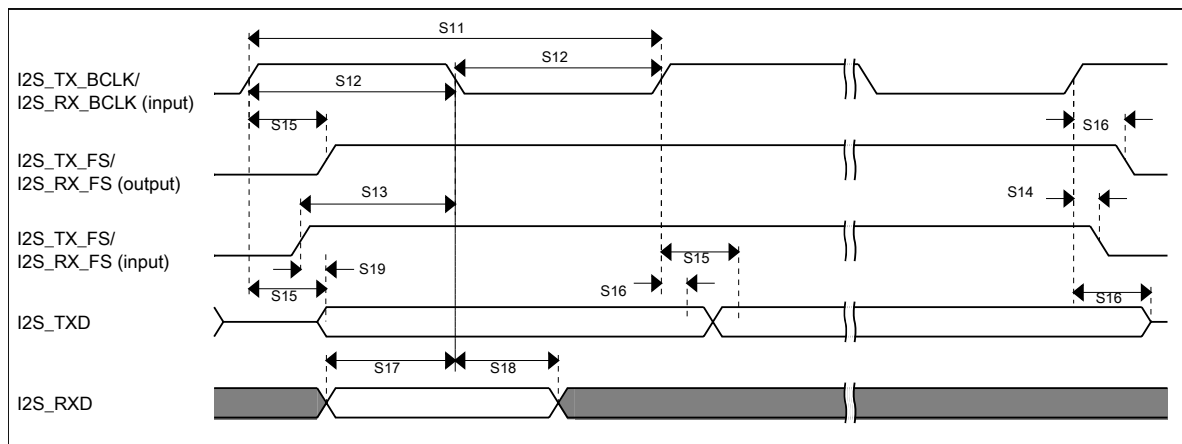
Figure 41. I2S/SAI timing — slave modes
