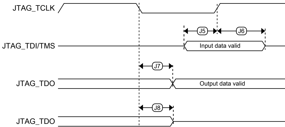
Figure 8. Boundary scan (JTAG) timing
