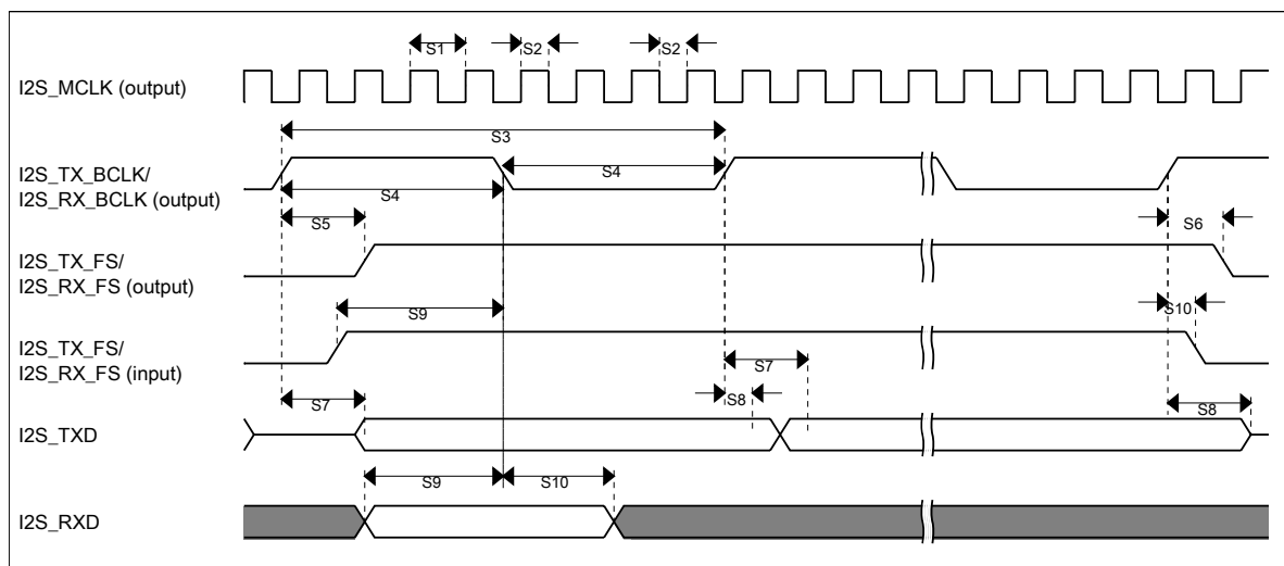
Figure 40. I2S/SAI timing — master modes
