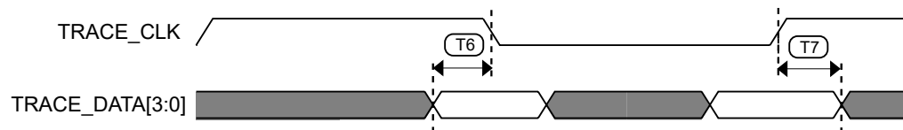
Figure 6. Trace data specifications
