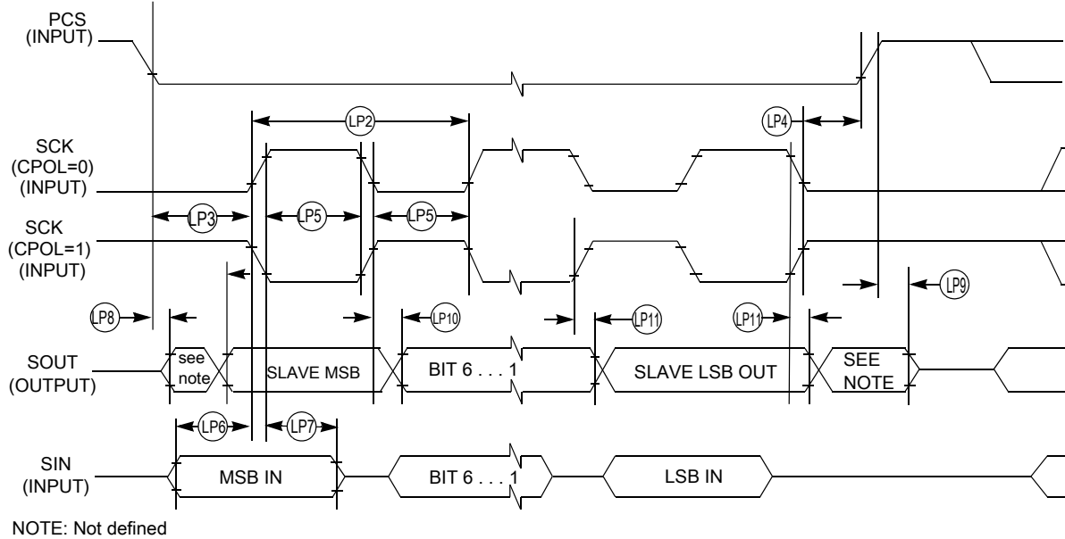
Figure 32. LPSPI slave mode timing (CPHA = 0)
