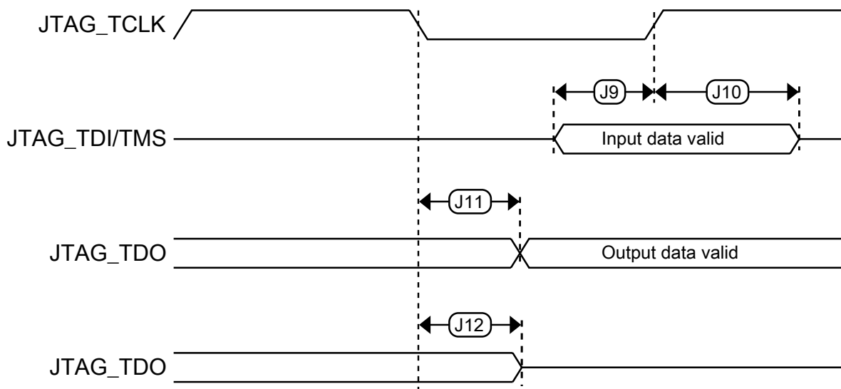
Figure 9. JTAG-DP/TAP timing
