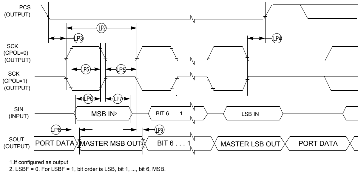
Figure 31. LPSPI master mode timing (CPHA = 1)
