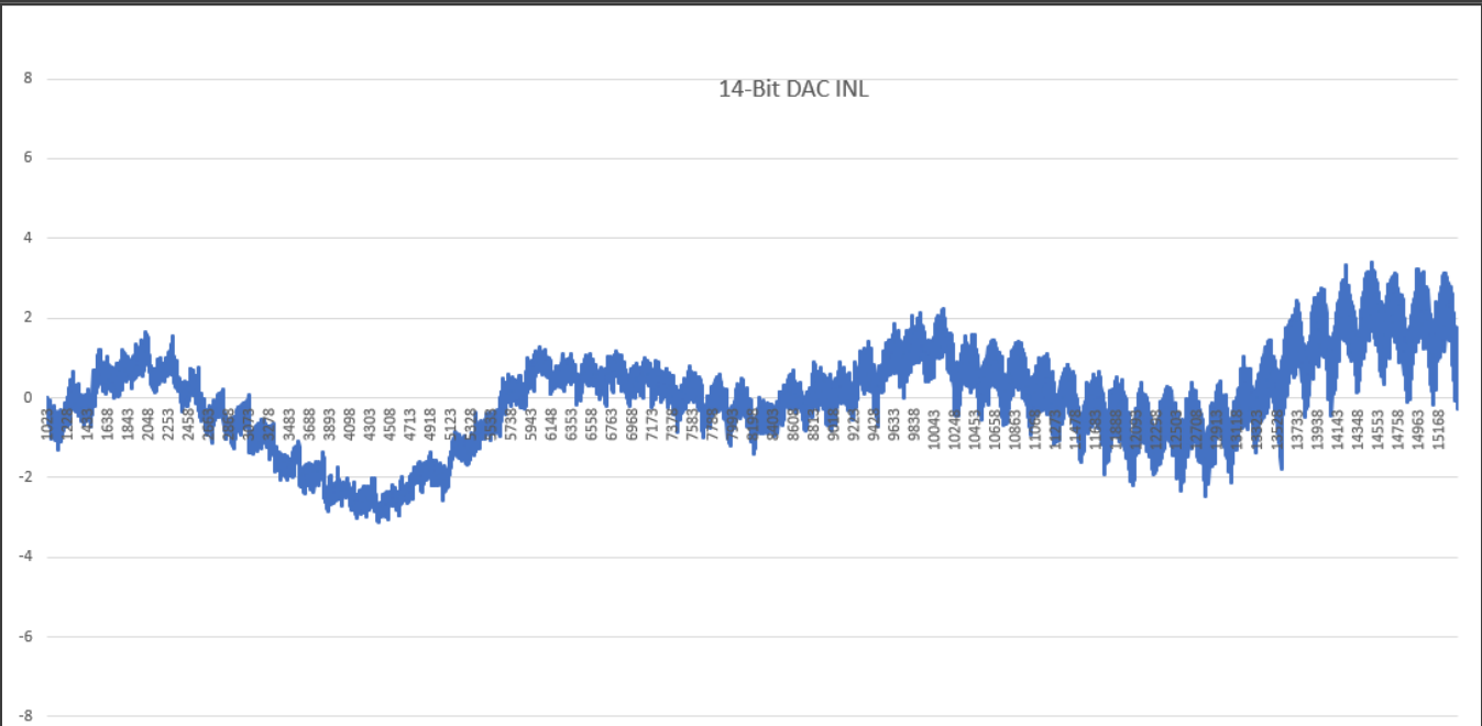
Figure 26. 14-bit DAC INL
