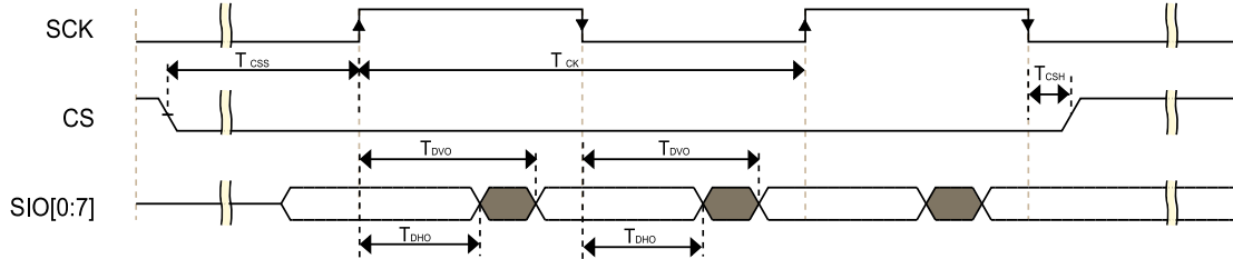
Figure 20. FlexSPI output timing in DDR mode
