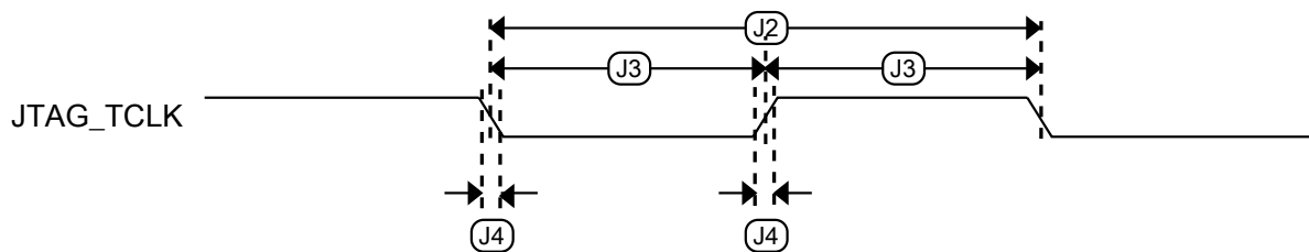
Figure 7. Test clock input timing
