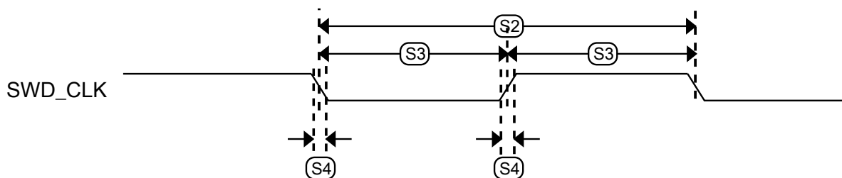
Figure 10. Serial wire clock input timing
