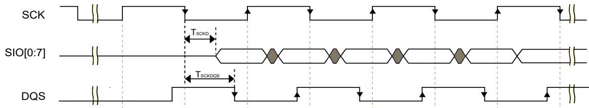
Figure 17. FlexSPI input timing in DDR mode where FlexSPI n _MCR0[RXCLKSRC] = 0x3 (case B1)
