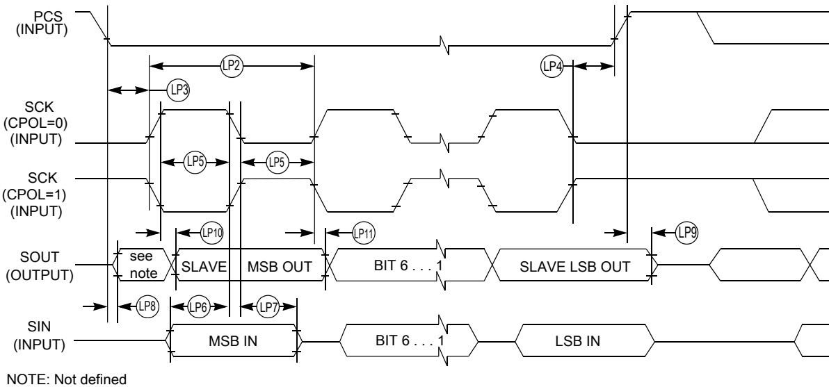
Figure 33. LPSPI slave mode timing (CPHA = 1)
