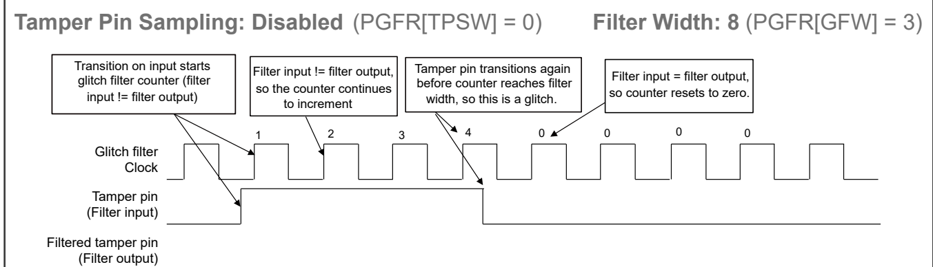
Figure 86. Tamper pin glitch filtering example: glitch
