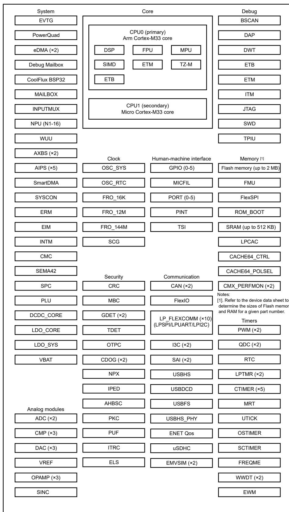
Figure 2. Features block diagram
