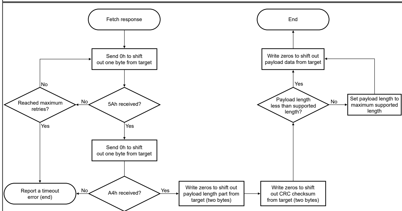
Figure 32. Host reads response from target via SPI
