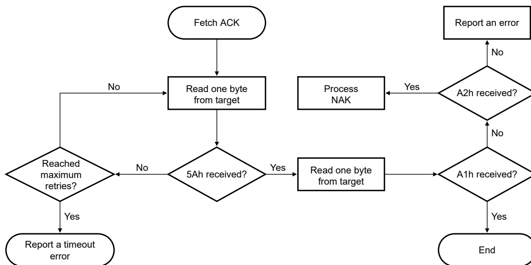
Figure 27. Host reads ACK packet from target via I 2 C
