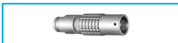
PHG.2B.514 Free socket, key (G) or keys (A...M), cable collet and nut for fitting a bend relief
