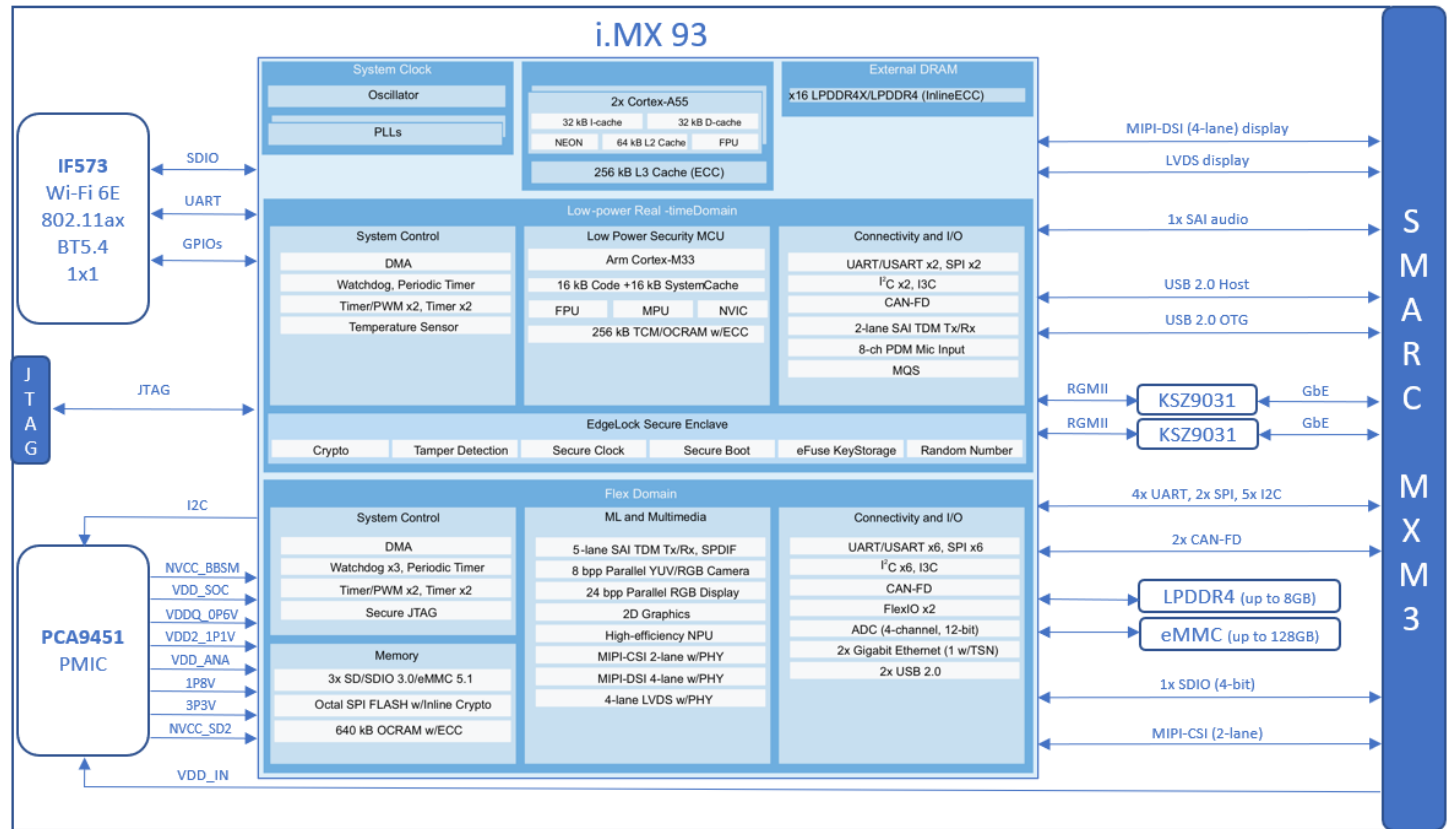
Figure 1: Nitrogen93 SMARC block diagram
