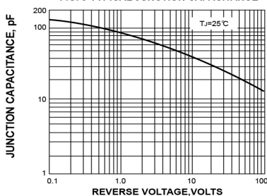
FIG. 5-TYPICAL JUNCTION CAPACITANCE
