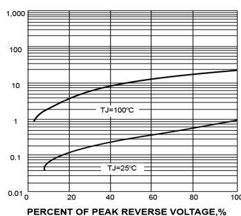
FIG. 4-TYPICAL REVERSE CHARACTERISTICS
