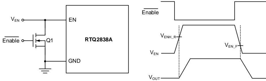
Figure 9. Logic Control for the EN Pin
