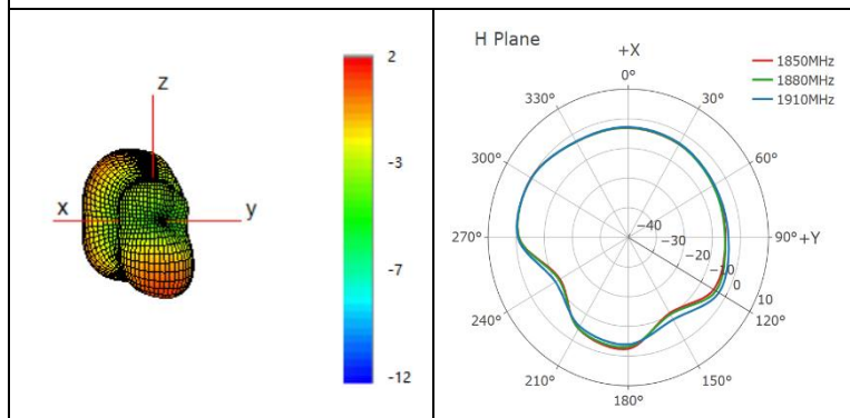
1880 MHz
