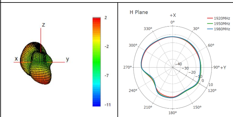
1950 MHz
