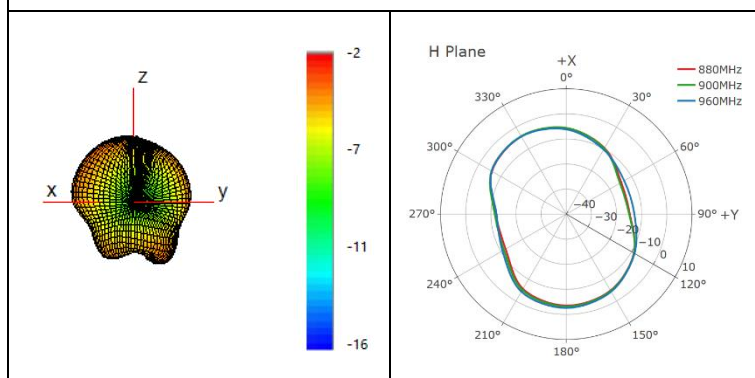
900 MHz
