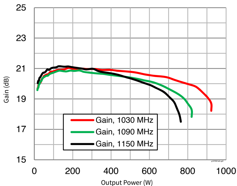
Figure 2. Power Sweep: Gain vs Output Power (Series Show Gain at Frequency) V_{DS} = 50 V, I_{DQ} = 100 mA, 128 \mu s Pulse Width, 10% Duty Cycle, Power Optimized
