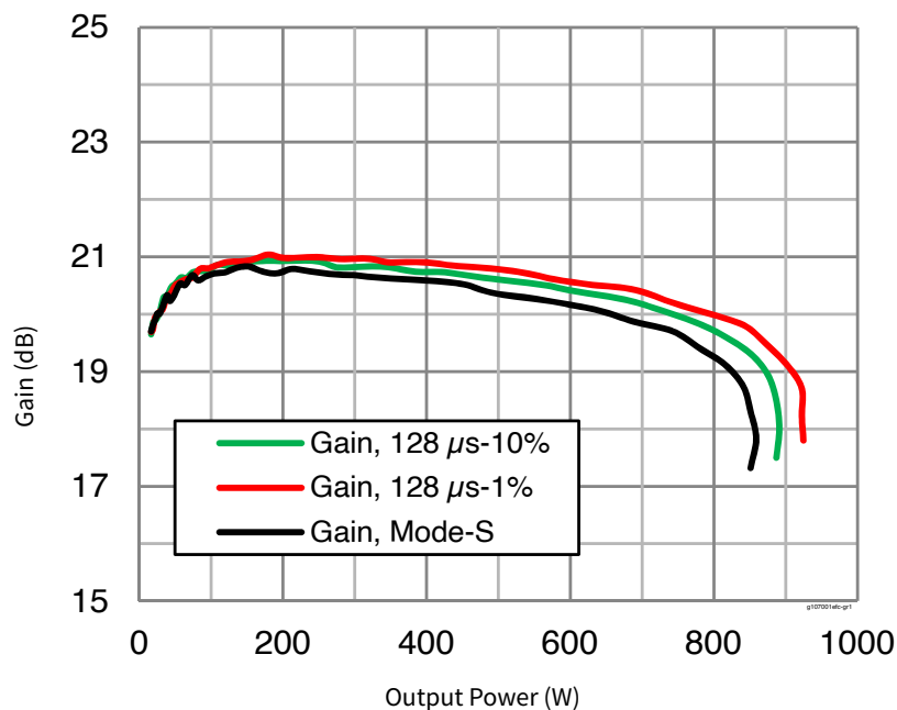
Figure 3. Power Sweep: Gain vs Output Power (Series Show Gain at Various Duty Cycles) V_{DS} = 50 V, I_{DQ} = 100 mA, f = 1030 MHz
