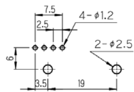
Circuit board hole dimension (View of solder surface)
