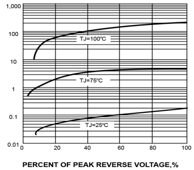
FIG. 4-TYPICAL REVERSE CHARACTERISTICS
