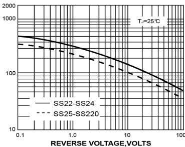
FIG. 5-TYPICAL JUNCTION CAPACITANCE
