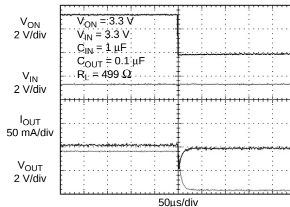
Figure 19. FPF1007 Turn-Off Response
