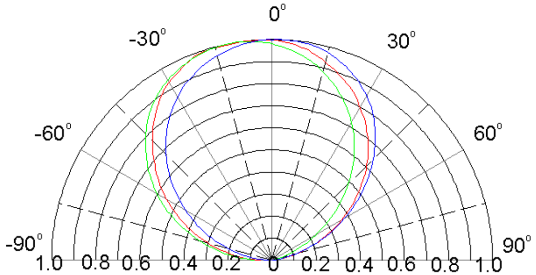
Figure5. Relative Luminosity VS. Radiation Angle
