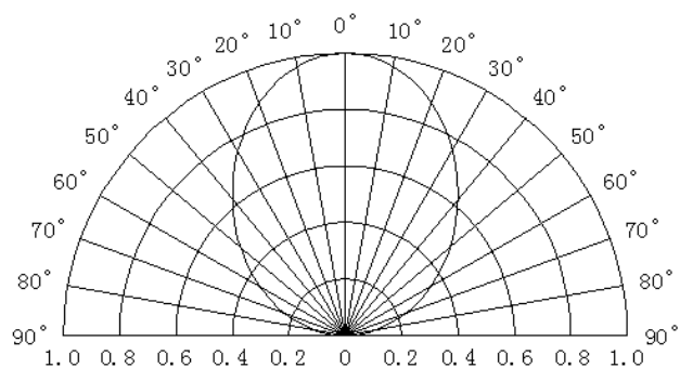
Relative Luminosity VS. Radiation Angle
