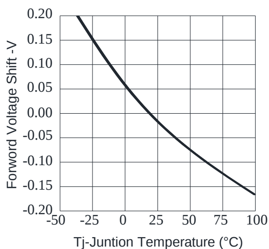
Fig.5-Forwd Voltage Shift vs. Juntion Temperature
