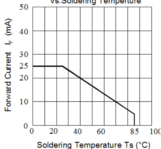
Fig.4-Max.Driving Forward Current vs.Soldering Temperature
