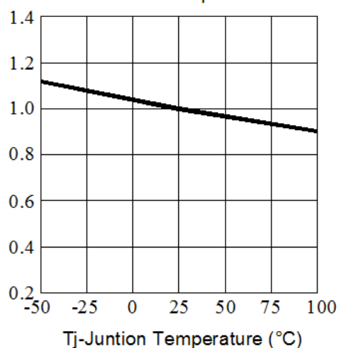
Fig.3-Relative Luminous Intensity vs.Juntion Temperature
