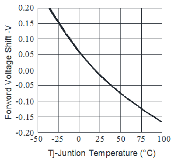
Fig.5-Forward Voltage Shift vs. Juntion Temperature
