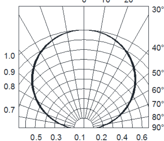
Fig.6-Radiation Diagram Ta=25°C
