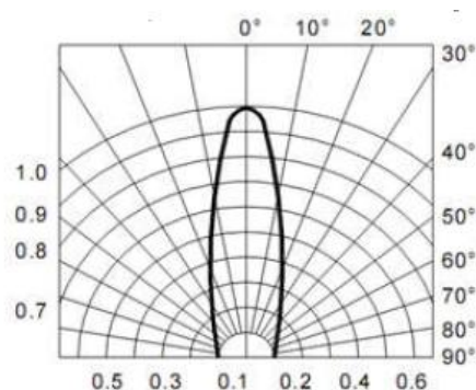
Relative Luminosity VS. Radiation Angle
