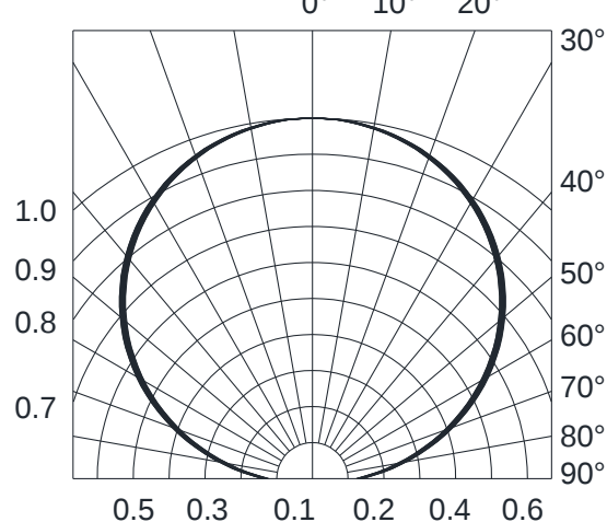
Fig.6-Radiation Diagram Ta=25°C
