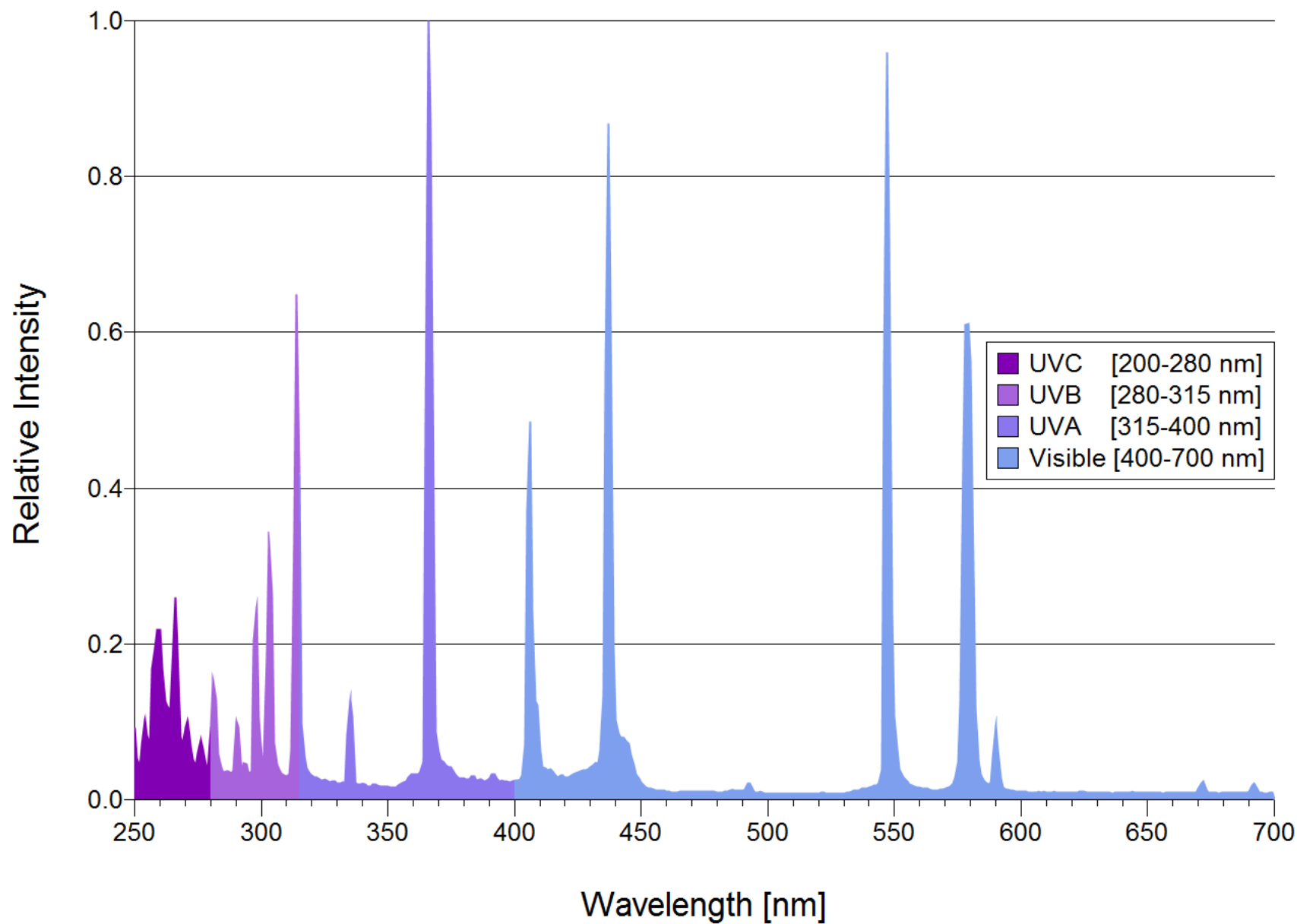
Uvitron 600W UVB Lamp Spectral Distribution UV1884
