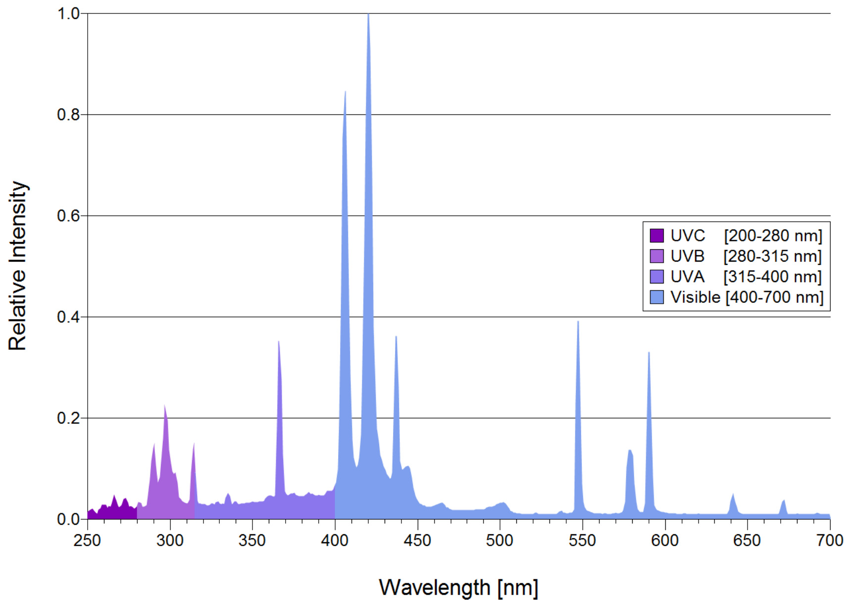
Uvitron 600W Visible Enhanced Lamp Spectral Distribution (420 nm ctr) UV1074
