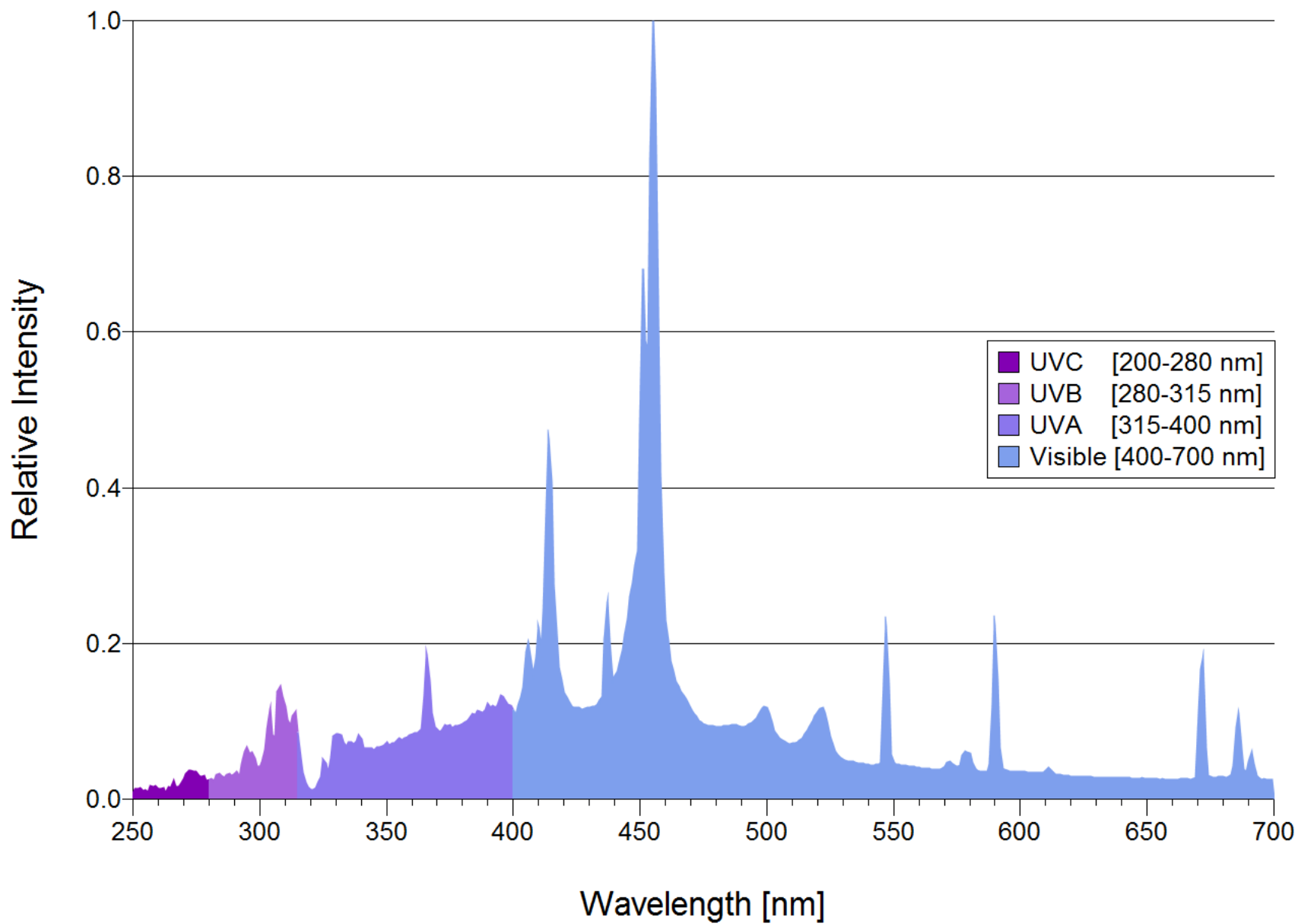
Uvitron 400W Visible Enhanced Lamp Spectral Distribution (460 nm ctr) UV0545
