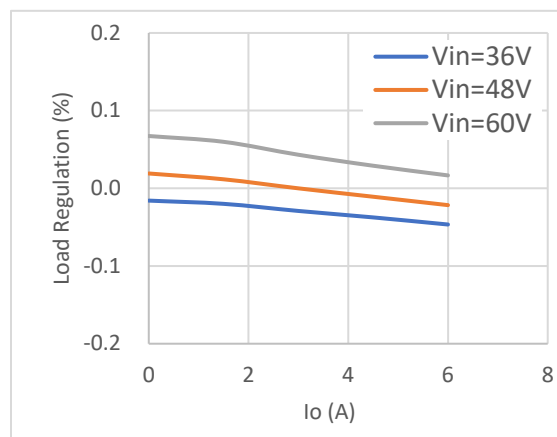
Load Regulation
