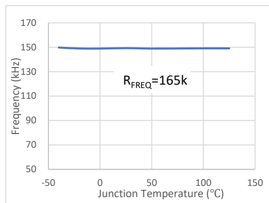
Frequency vs. Junction Temperature
