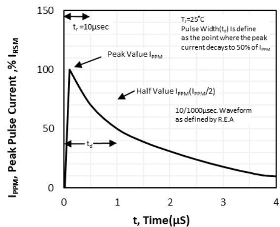
Figure 4 10/1000 \mu\text{s} Pulse Waveform
