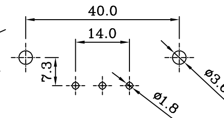
FRONT MOUNTING
