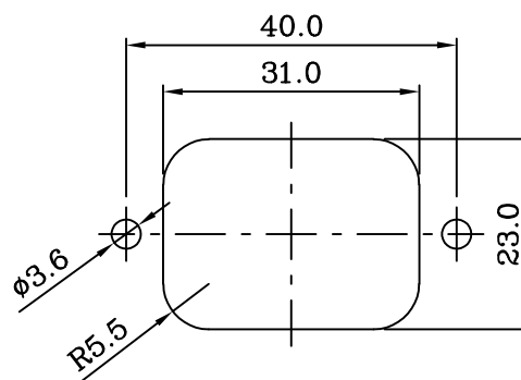
REAR MOUNTING
