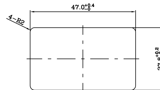
PANEL CUT-OUT
