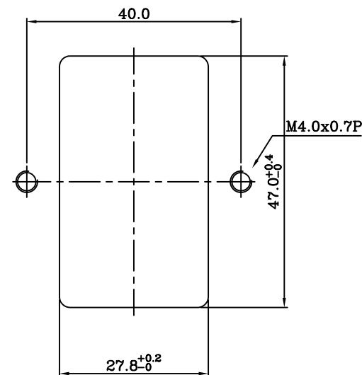
PANEL CUT-OUT
