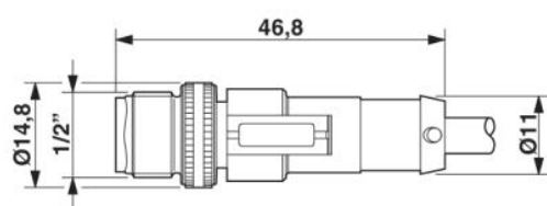
1/2"-20UNF plug, straight
