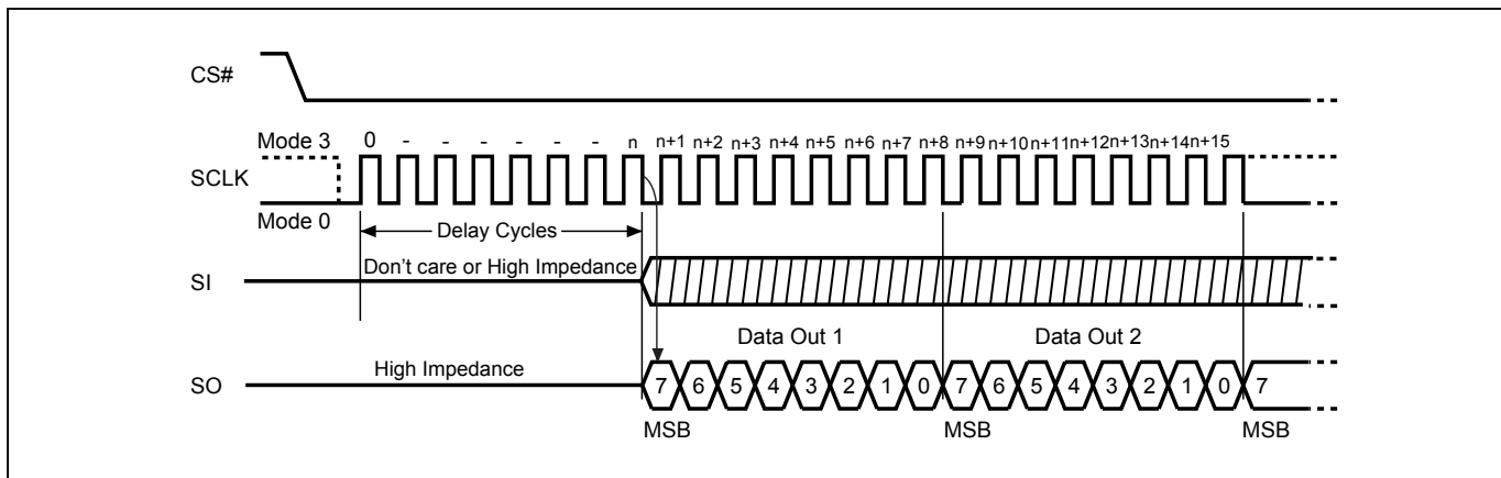
Figure 67. Fast Boot Sequence (QE=0)
