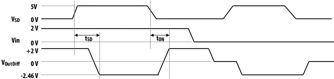
Figure 17: Shutdown And Wakeup Input To Output Timing Diagram. V_{Out\ Diff} = V_{Out+} - V_{Out-}
