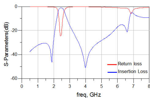
RFBPF2012090A2T
