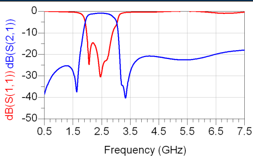
RFBPF2012100AVT
