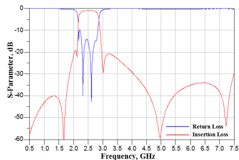
RFBPF2012090A2T
