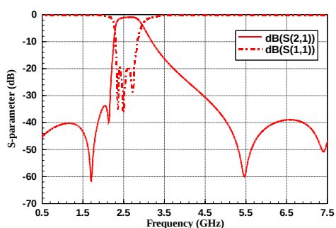
RFBPF2012090A1T
