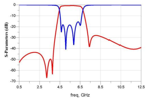
RFBPF2012090K5T
