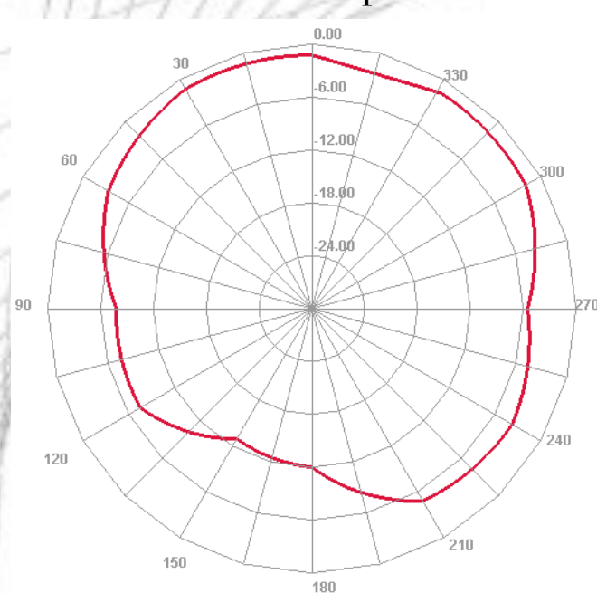
900MHz H plane
