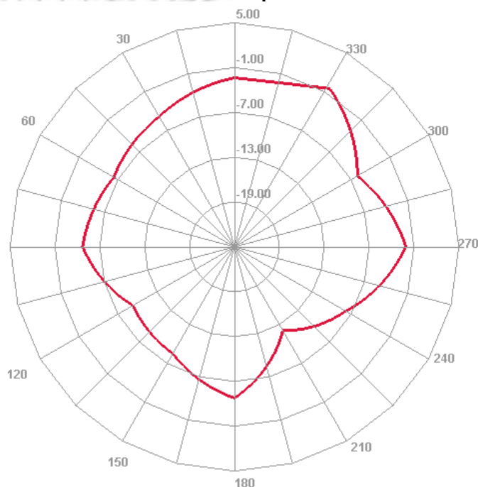
4800MHz H plane
