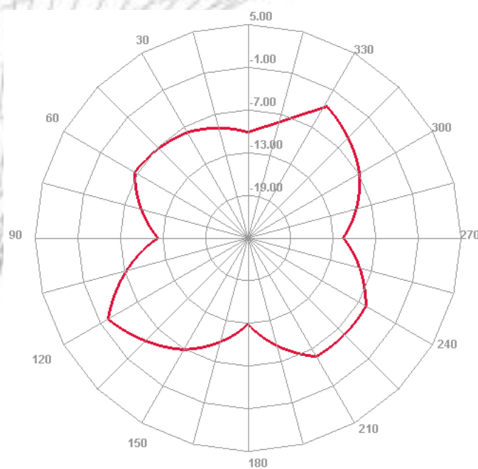
5800MHz H plane
