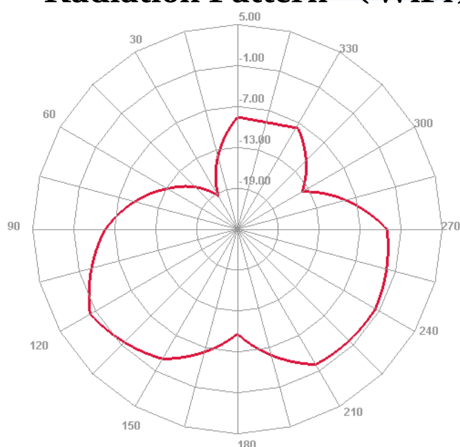
2400 MHz E plane
