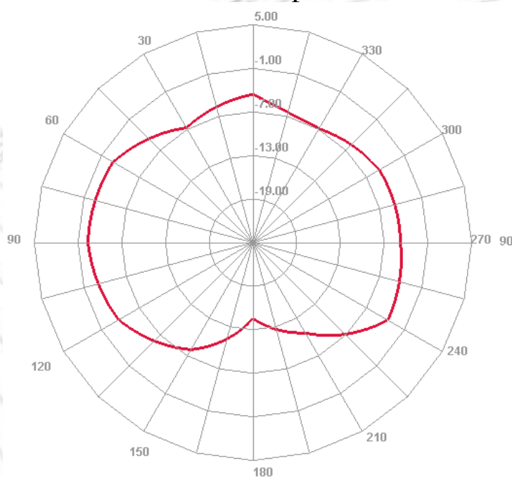
4800MHz E plane
