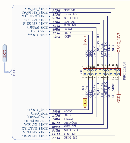
EXT2 Extension Header
