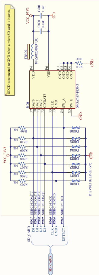
microSD-CARD
