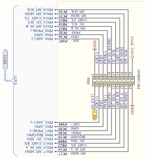
EXT1 Extension Header
