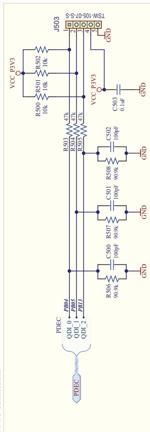
PDEC Connections
