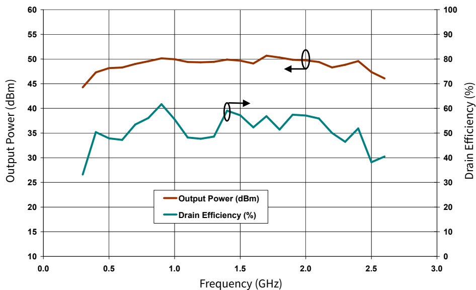
Figure 2. Output Power and Drain Efficiency vs Frequency Measured in Broadband Amplifier Circuit CGH40090PP-AMP V_{DD} = 28 V, I_{DQ} = 1.0 A
