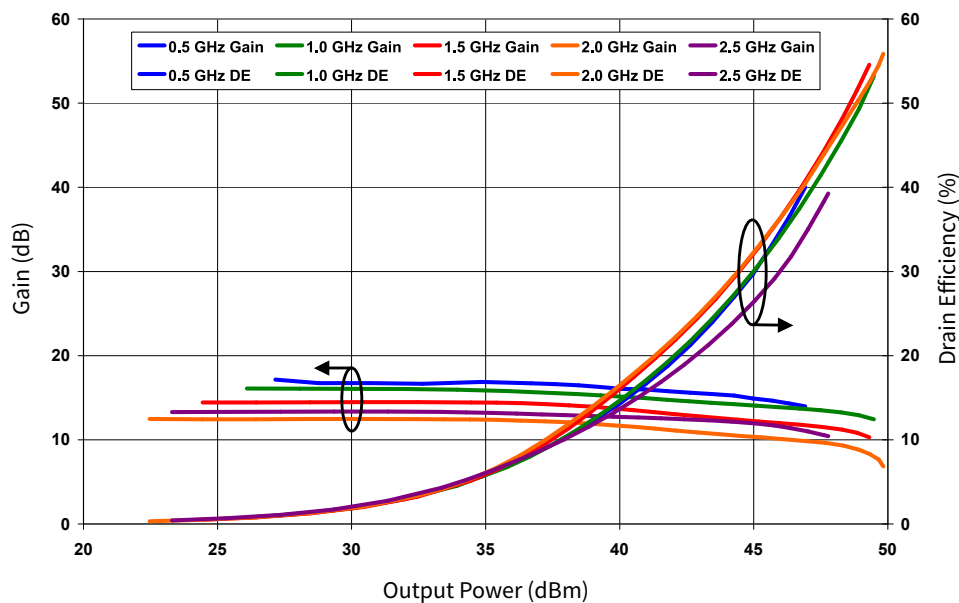
Figure 1. Gain and Efficiency vs Output Power Measured in Broadband Amplifier Circuit CGH40090PP-AMP V_{DD} = 28 V, I_{DQ} = 1.0 A, Freq = 0.5 - 2.5 GHz
