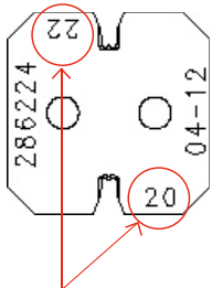
Switch wire crimper and insulation crimper die according to the wire size being used.
