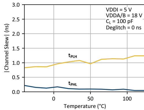
Figure 27. Channel-to-Channel Skew vs. Ambient Temperature
