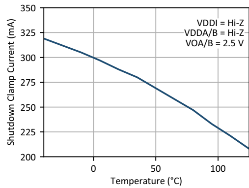
Figure 39. Shutdown Clamp Current vs. Ambient Temperature
