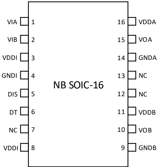
Figure 1. Si82D29x Pinout
