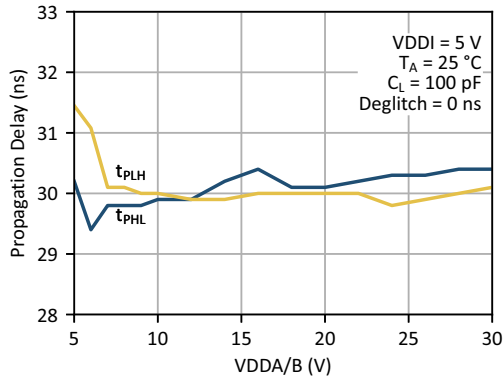
Figure 24. Propagation Delay vs. Gate Driver Supply Voltage
