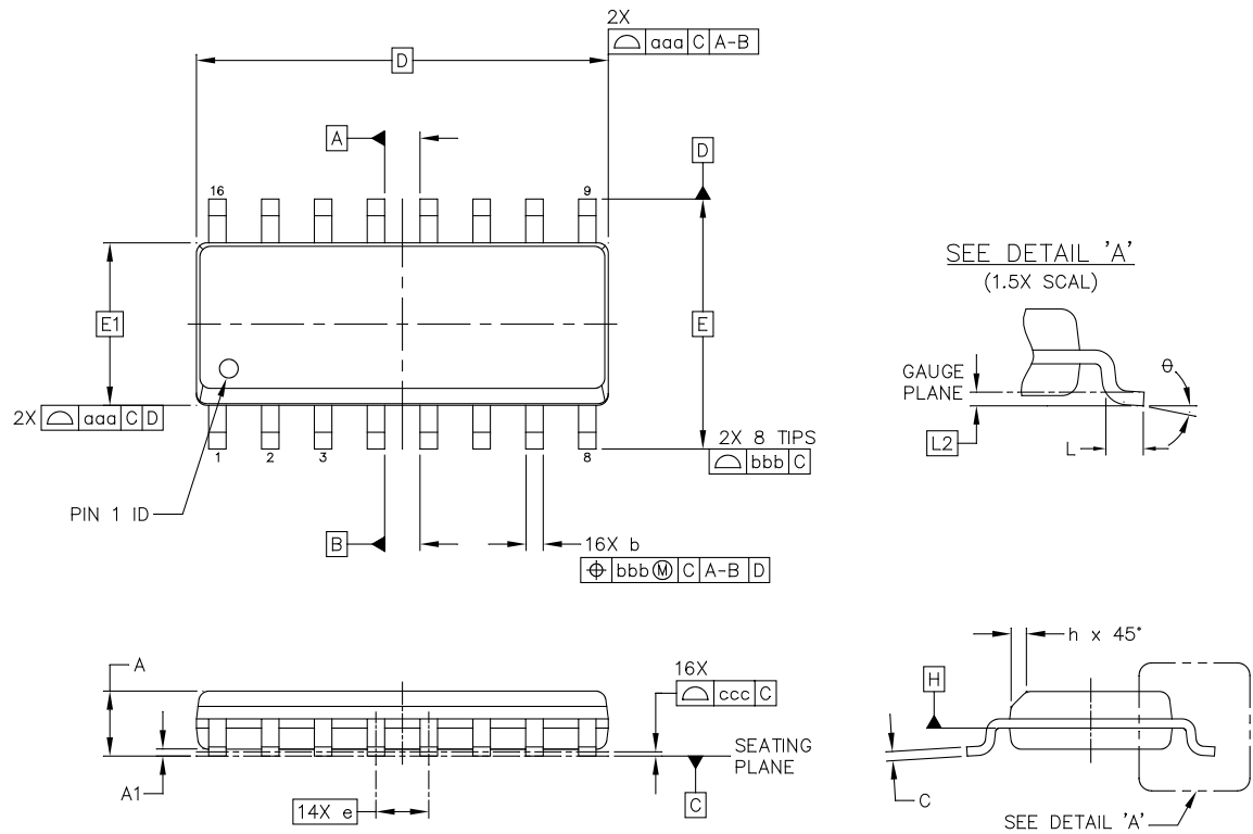
Figure 42. NB SOIC-16 Package Drawing
