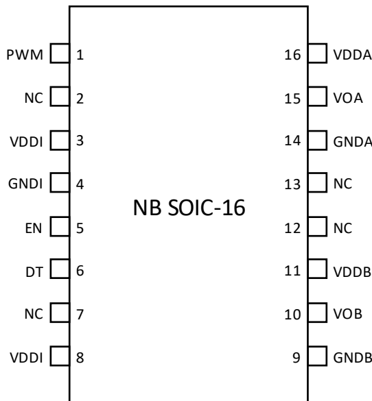
Figure 4. Si82D99x Pinout
