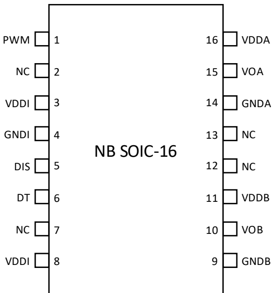
Figure 3. Si82D89x Pinout
