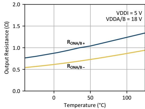
Figure 37. Output Resistance vs. Ambient Temperature
