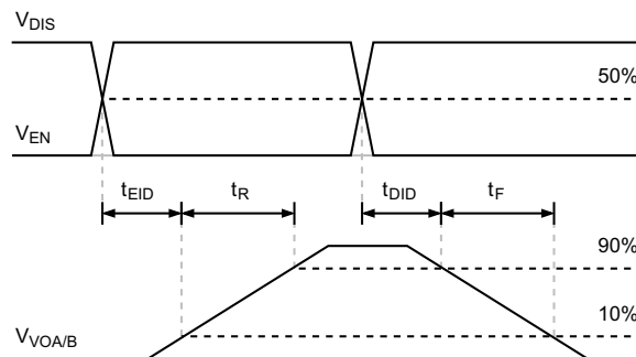
Figure 21. Enable or Disable Input Timing Measurements
