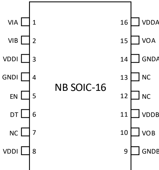
Figure 2. Si82D39x Pinout
