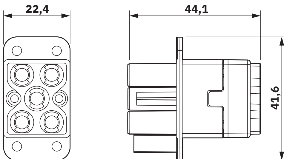
Dimensional drawing
