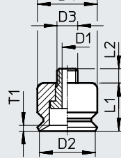
ESS-150/200-S
