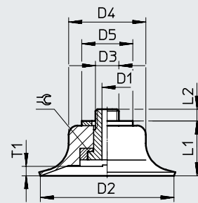
ESS-40/50/60-S
