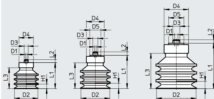
ESS-10-C
