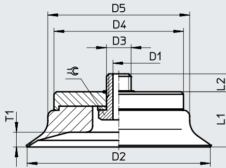
ESS-150/200-S
