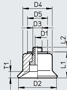
ESS-20/30-S
