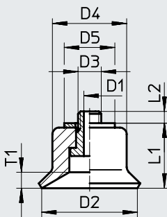
ESS-20/30-E
