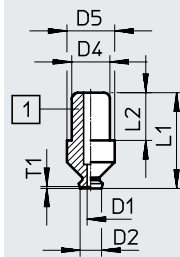
ESS-80/100-S
