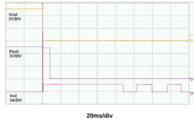
Figure 8. Extended Short-Circuit into Thermal Cycles
